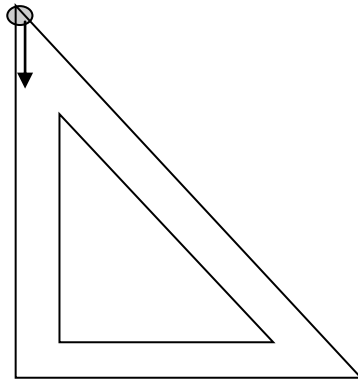
triangle -rectangle
