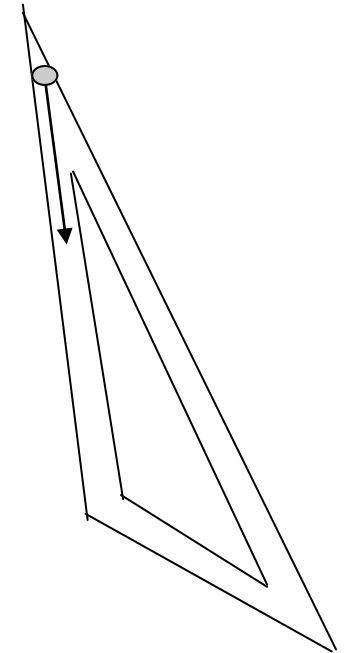
triangle quelconque
